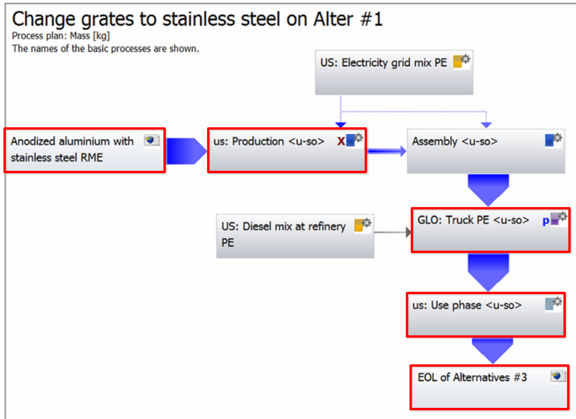
Figure 7.9 Simulation of LCA framework on alternative #3
