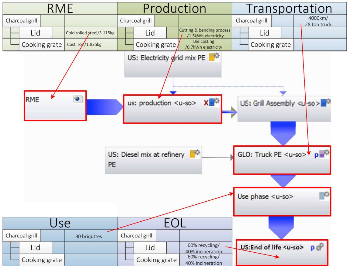
Figure 7.6 Use LCA to simulate LCAatPLM with an example
