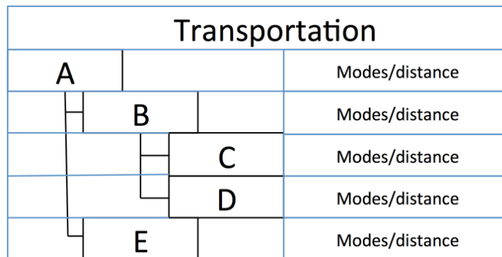
Figure 5.5 Transportation in proposed LCA framework
