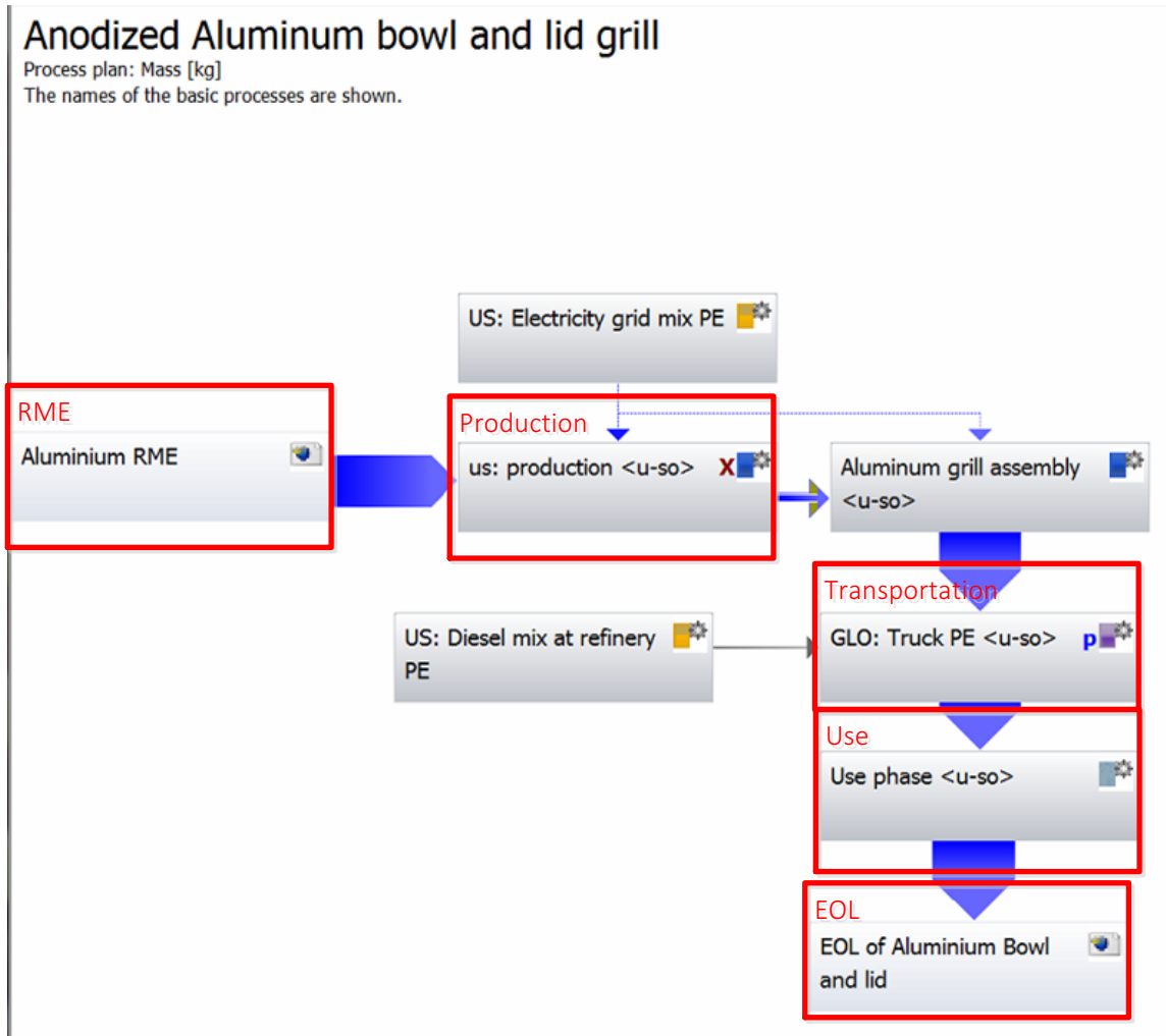
Figure 7.1 Simulation of LCAatPLM
