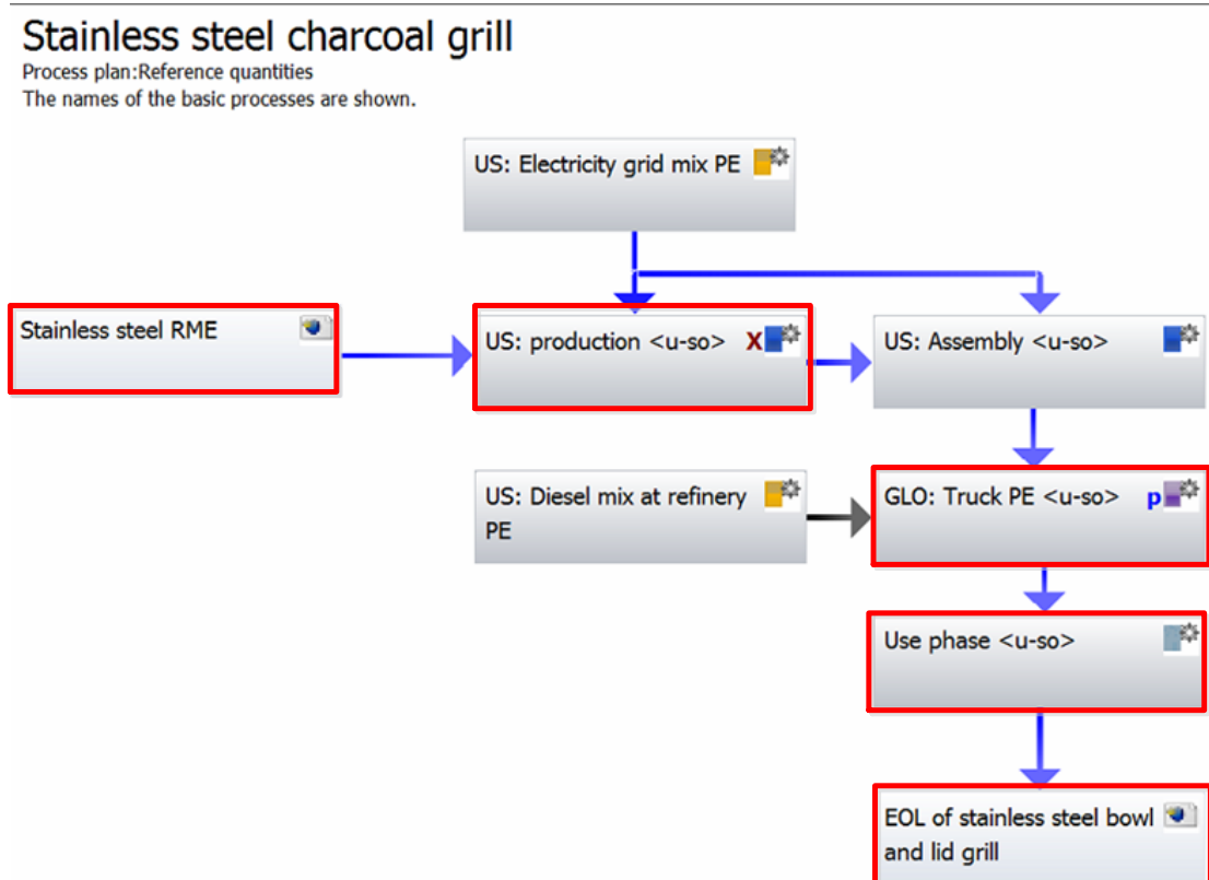
Figure 7.8 Simulation of LCA framework on alternative #2
