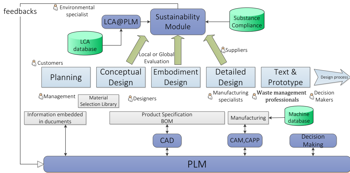
Figure 5.9 Proposed system architecture
