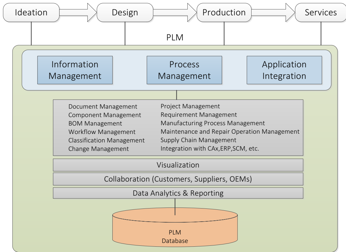
Figure 2.1 PLM architecture
